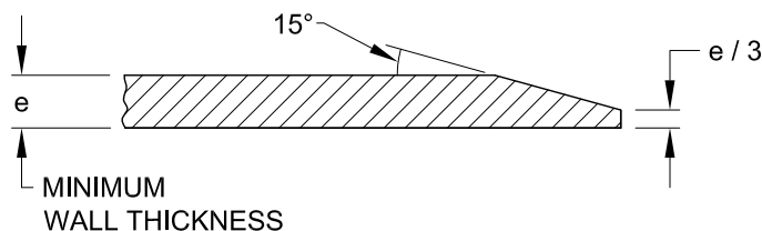
FIG. 6 PIPE ENDS
